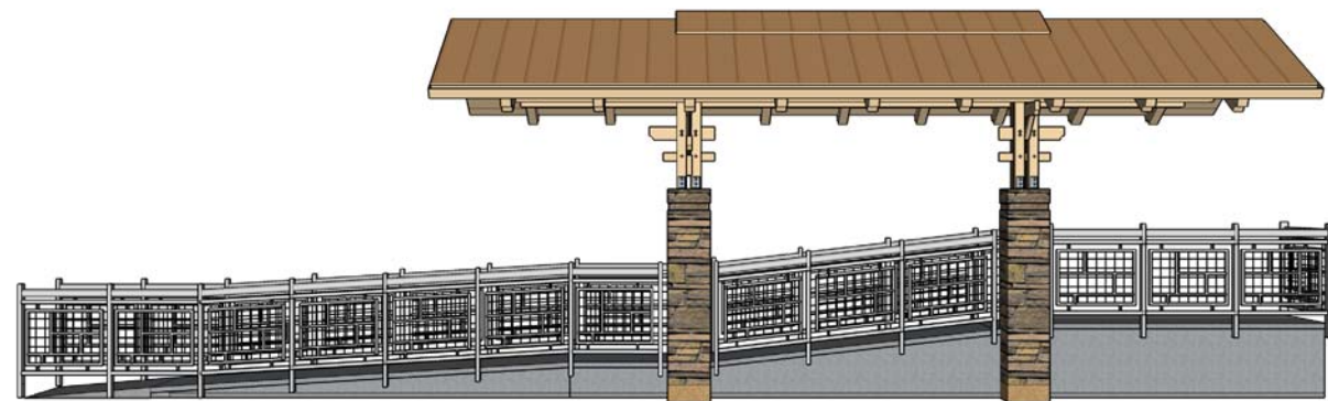
HIGHBLOCK FRONT ELEVATION
