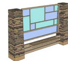
WINDSCREEN AXONOMETRIC VIEW
