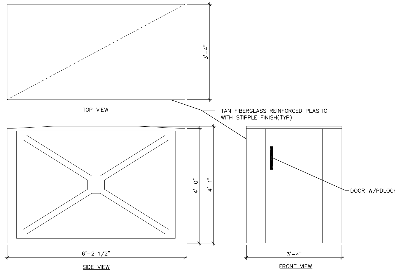
3 BICYCLE LOCKERS AMERICAN BICYCLE SECURITY MODEL 352 SCALE: 1"=1'-0" W/PADLOCK HANDLE PN #010
