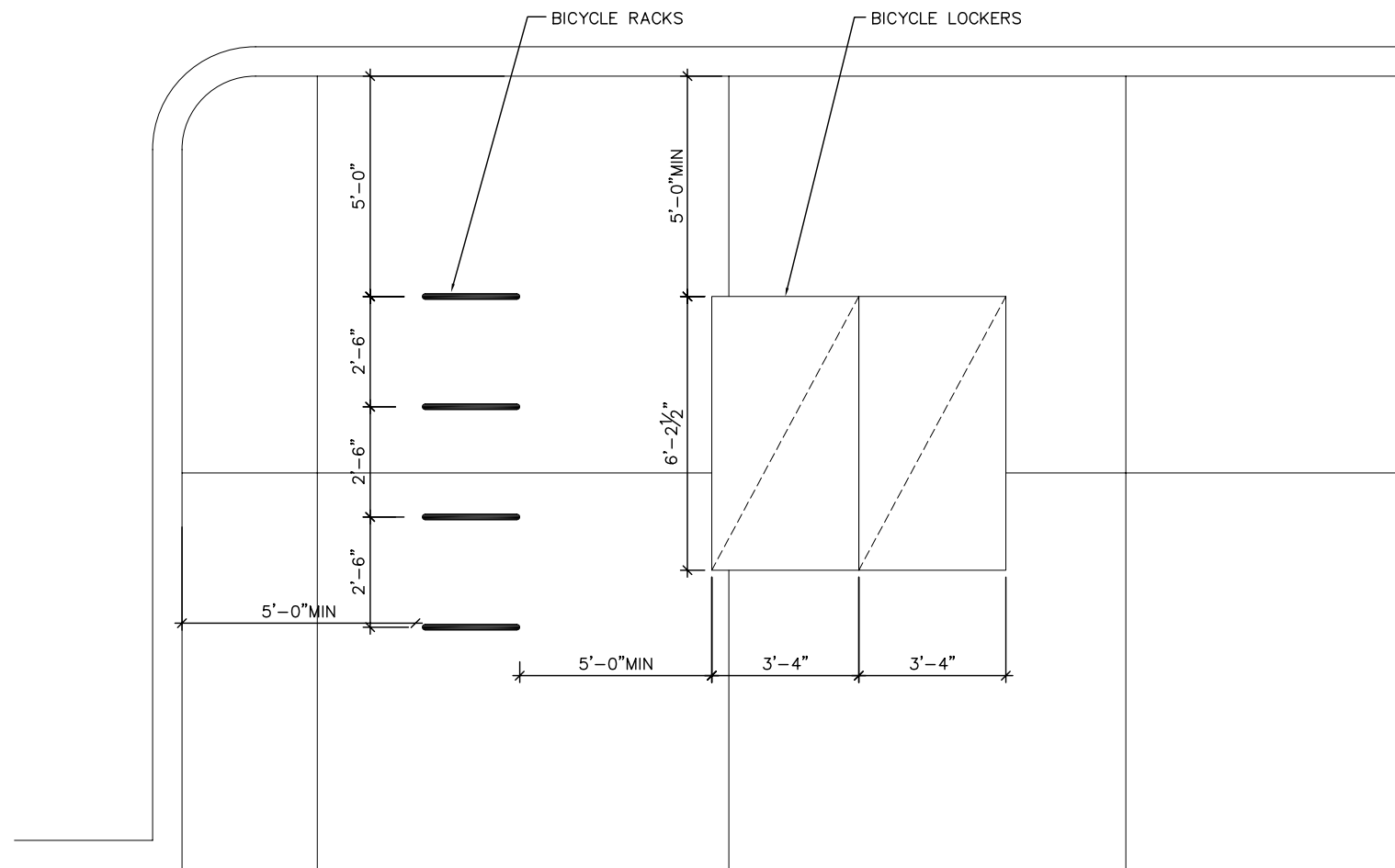
4 TYPICAL BICYCLE RACK & LOCKER LAYOUT SCALE: 1"=2'-0"
