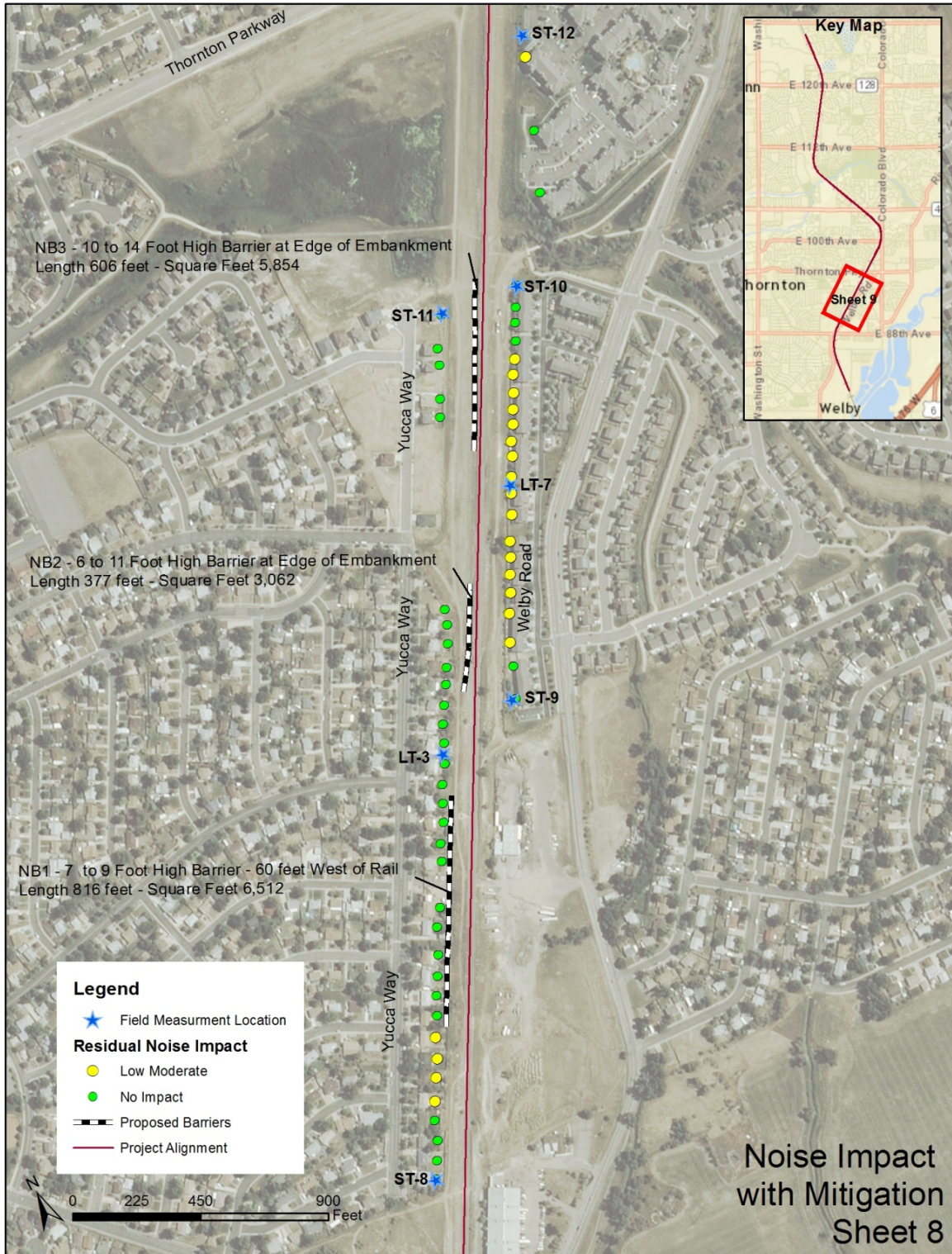
Figure 1-17. Final Alignment-Post Mitigation
