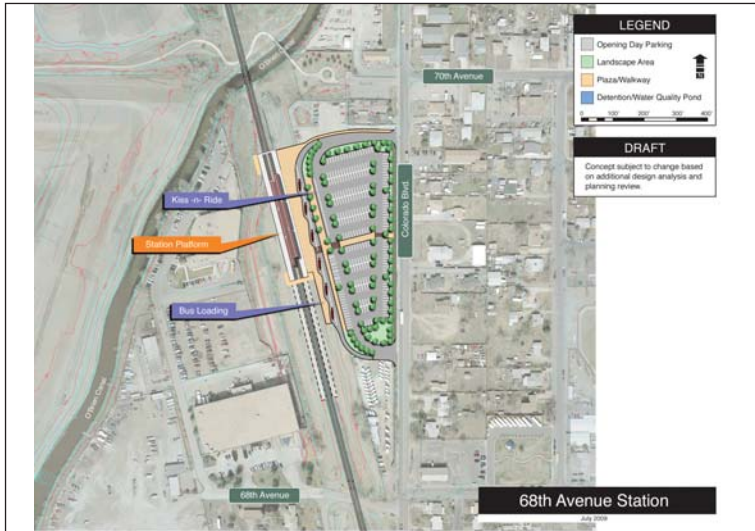
COMMERCE CITY 68 TH AVENUE STATION CONCEPT
