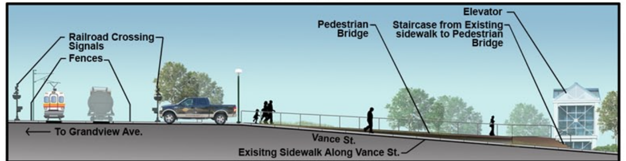
Section B-B
