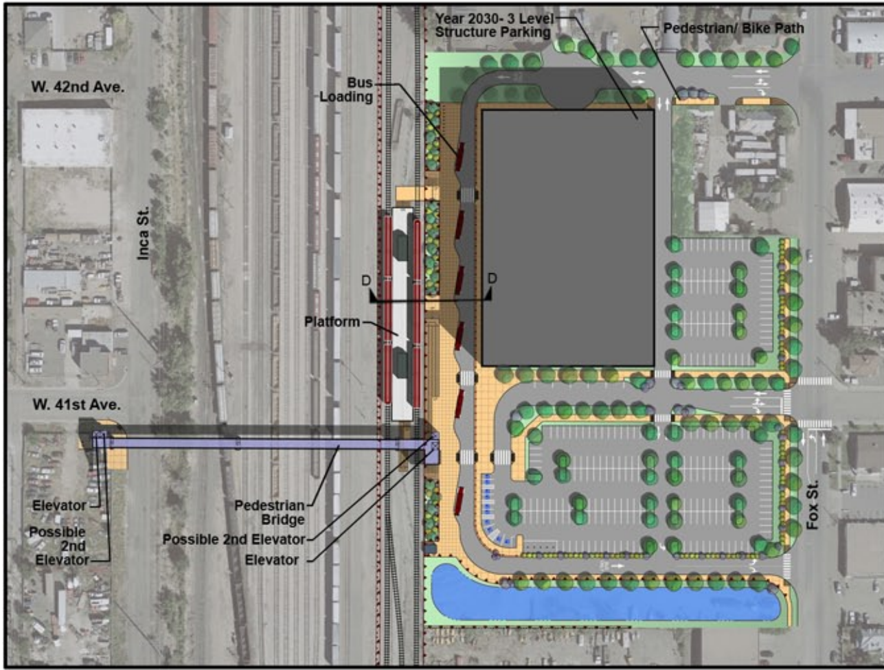
Site Plan (2030)
